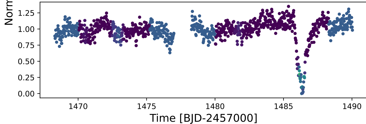
Single Model Predictions - Beta Pic
