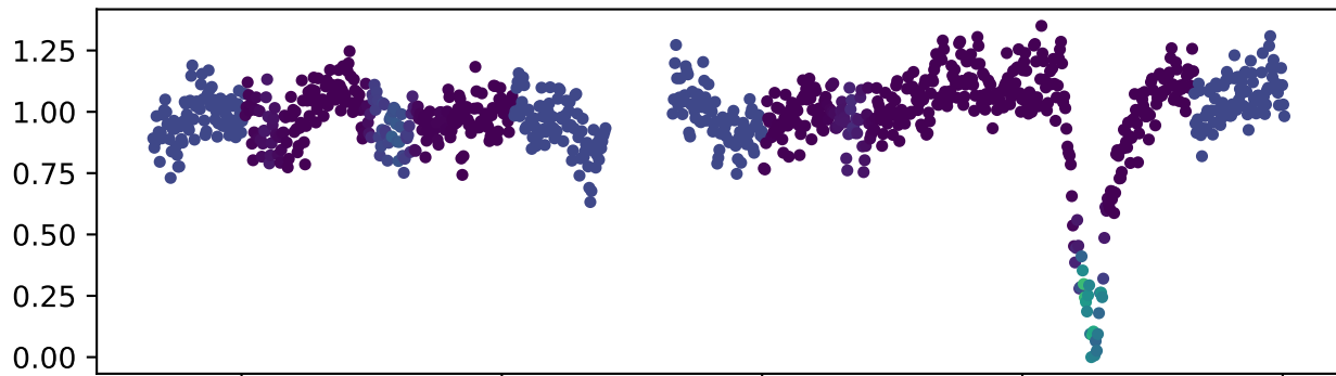
Single Model Predictions - Beta Pic
